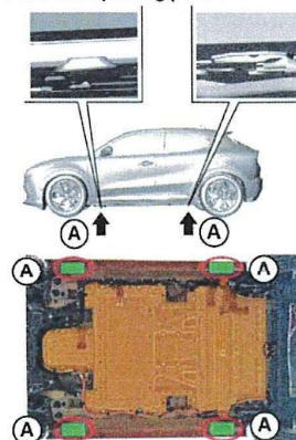
Stabilization/lifting points
